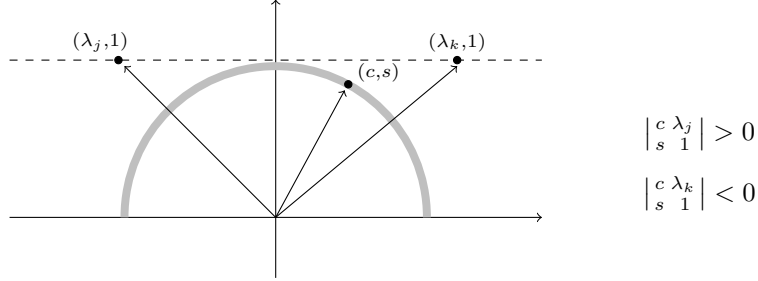
Figure 3.2: Pictorial representation of (3.2).
