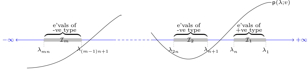
Figure 3.3: Distribution of eigenvalue types of n \times n hyperbolic polynomials of even degree m .
