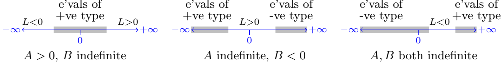
Figure 3.1: Distribution of the eigenvalue types for three types of definite pencils L(\lambda) = \lambda A - B . On the shaded intervals L is indefinite.
