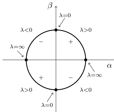
Figure 2.1: Correspondence between \lambda and (\alpha, \beta) .
