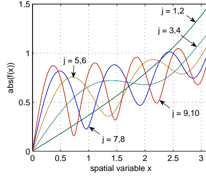
(b) absolute value of the 10 eigenfunctions found first (these are complex-valued)
