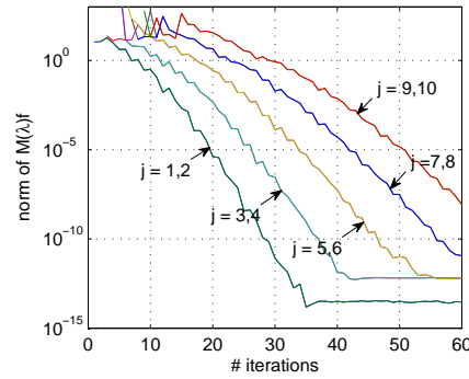
(d) residual norm \|\mathcal{M}(\lambda)f\| of the 10 eigenpairs (\lambda, f) found first, with curves coinciding pairwise
