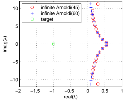
(a) approximate eigenvalues after 45 and 60 iterations of infinite Arnoldi, respectively
