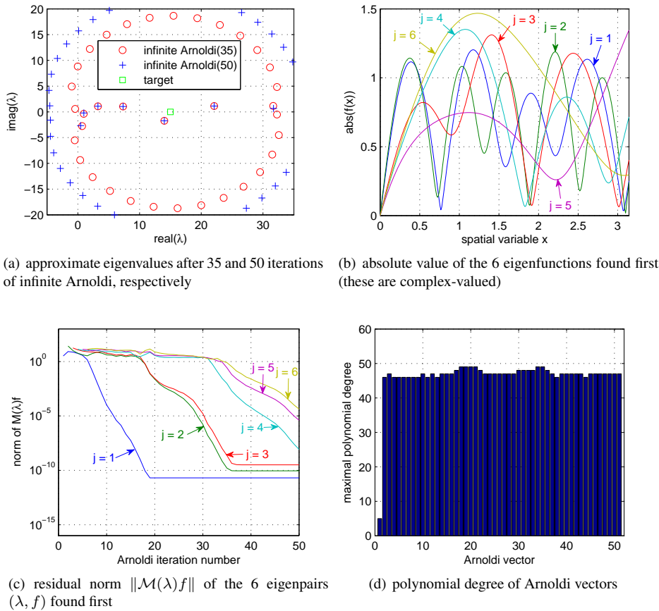
FIG. 4.3. The artificial example (Section 4.3)
