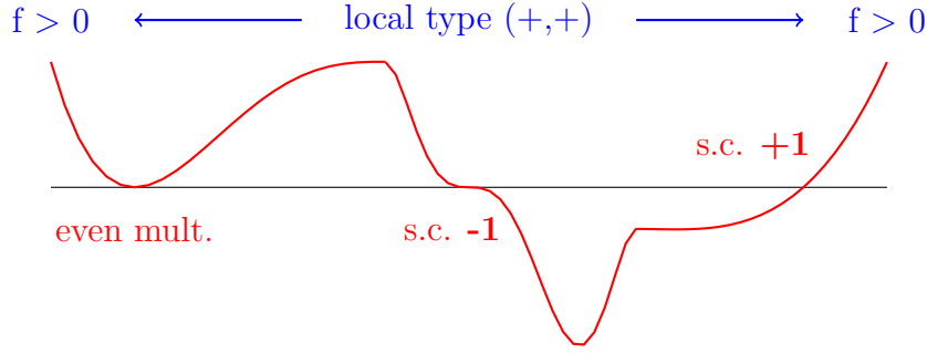
Figure 1: An analytic function f(x) having local type (+, +) in the interval \mathcal{J} .
